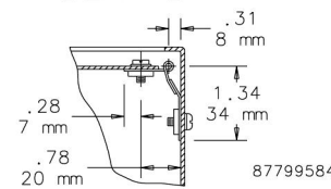
DETAIL X
